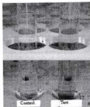
Photoplate 4: Arnow's Assay
