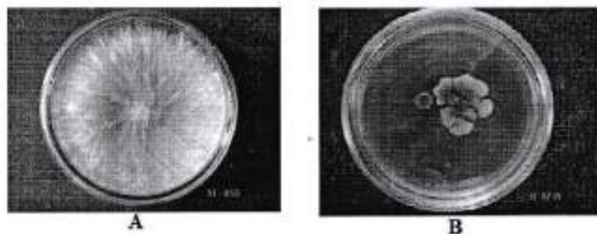
Photo Plate 1: Dual Culture technique of SMD against Sclerotium rolfii A) Control of Sclerotium rolfii B) SMD culture with Sclerotium rolfii
