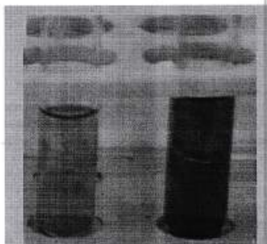
Photo Plate 2: Liquid CAS Assay for Siderophore Production A) Test B) Control
